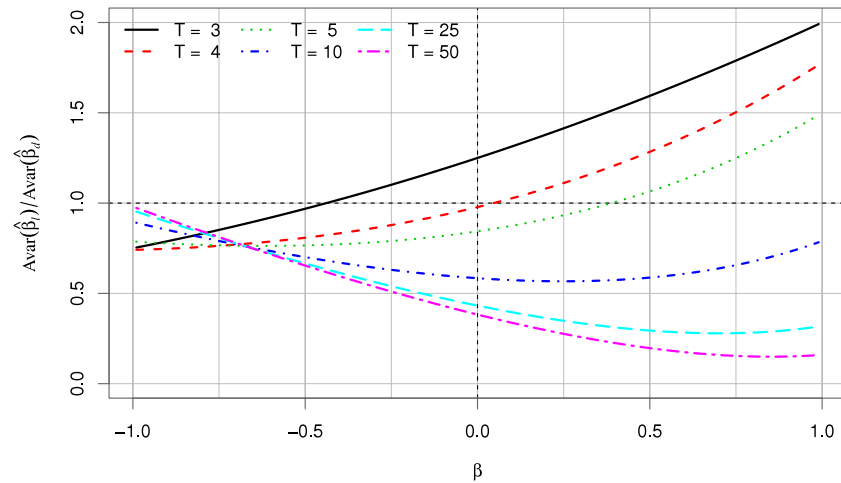
(b) \sigma_\alpha^2/\sigma^2 = 8 .
