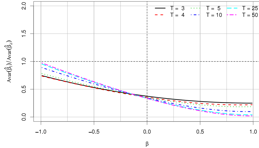
(a) \sigma_\alpha^2/\sigma^2 = 1 .
